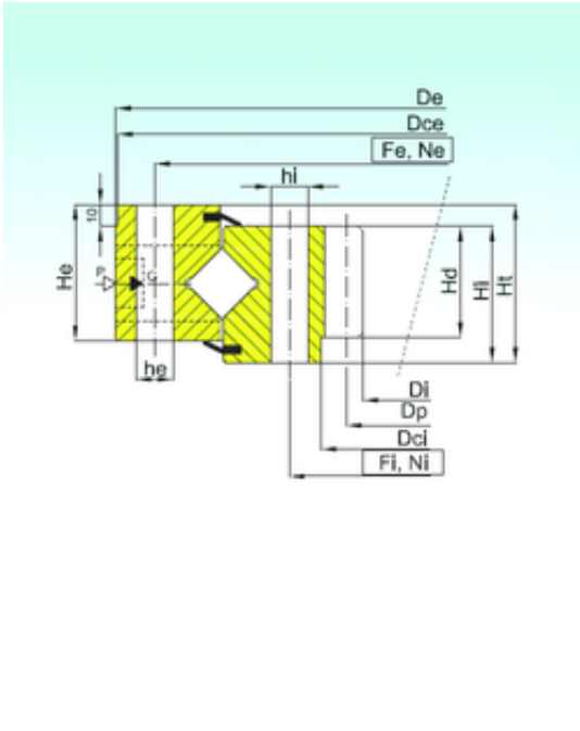
ZR1.16.0380.400-1SPPN Bearing 2D drawings and 3D CAD models
